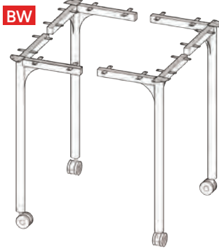
Fixed Height Leg (with lockable castors) 970 mm high
