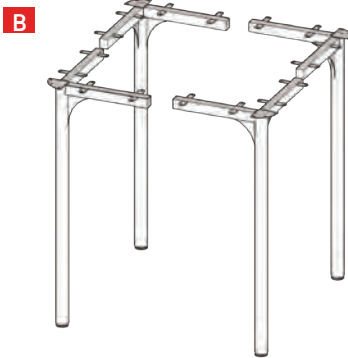
Fixed Height Leg (with levelling feet) 900 mm high
