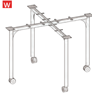
Fixed Height Leg (with lockable castors) 720 mm high
