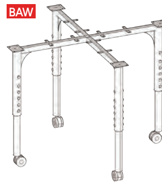
Fixed Height Adjustable Leg (with lockable castors) 6 heights: 720 | 780 | 810 | 850 | 900 | 930 mm
