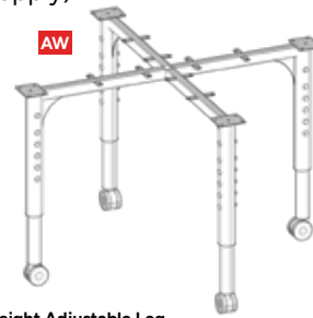
Height Adjustable Leg (with lockable castors) 6 heights: 550 | 610 | 640 | 680 | 720 | 750 mm
