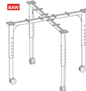
Height Adjustable Leg (with lockable castors) 6 heights: 720 | 780 | 810 | 850 | 900 | 930 mm
