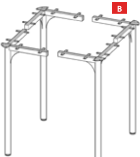
Fixed Height Leg (with levelling feet) 900 mm high
