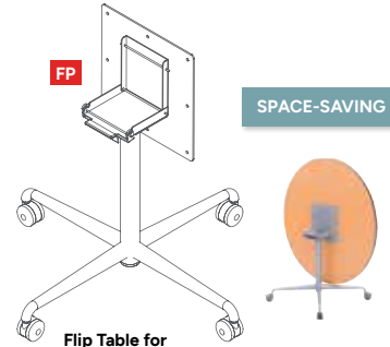
Flip Table for Easy Storage (with lockable castors) 720 mm high
